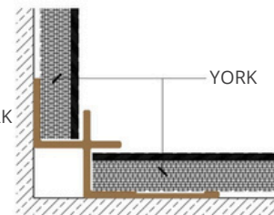
INTERNAL ANGLE PROFILE
