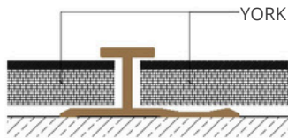
I PROFILE
