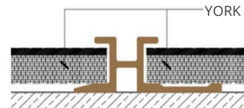
INNER CONCAVE PROFILE
